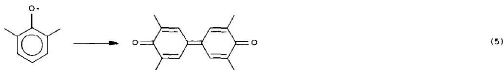
SCHEME I
